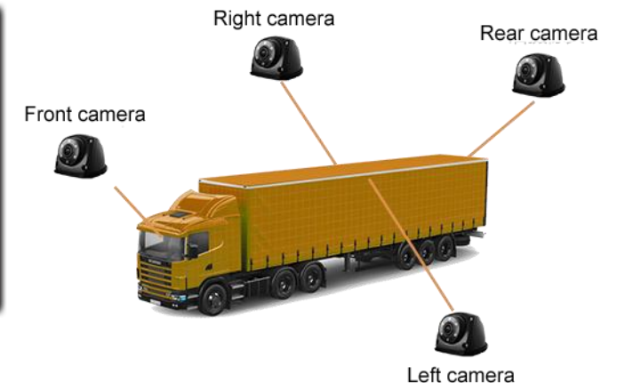
Panorama Stitching Solution Installation Diagram
